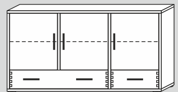
60282L/40/F/G* 134x70x40cm (BxHxT) 60282L/32/F/G* 134x70x32cm (BxHxT)
