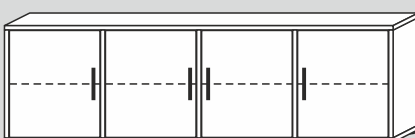
60343/40/F/G* 178x54x40cm (BxHxT) 60343/32/F/G* 178x54x32cm (BxHxT)
