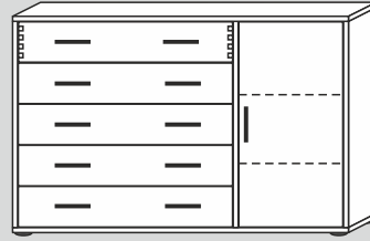
60301R/40/F/G* 134x86x40cm (BxHxT) 60301R/32/F/G* 134x86x32cm (BxHxT)
