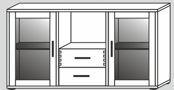
60278/40/F/G* 134x70x40cm (BxHxT) 60278/32/F/G* 134x70x32cm (BxHxT)
