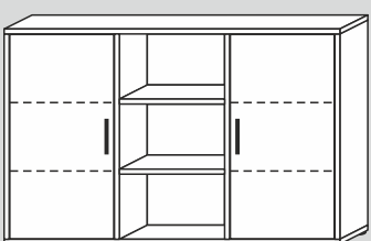
60292/40/F/G* 134x86x40cm (BxHxT) 60292/32/F/G* 134x86x32cm (BxHxT)
