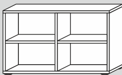
6086/40/F* 90x54x40cm (BxHxT) 6086/32/F* 90x54x32cm (BxHxT)
