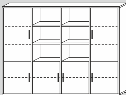
60659/40/F/G* 178x134x40cm (BxHxT) 60659/32/F/G* 178x134x32cm (BxHxT)
